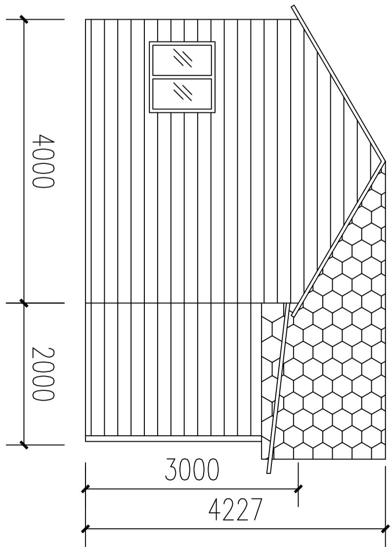
Left elevation
