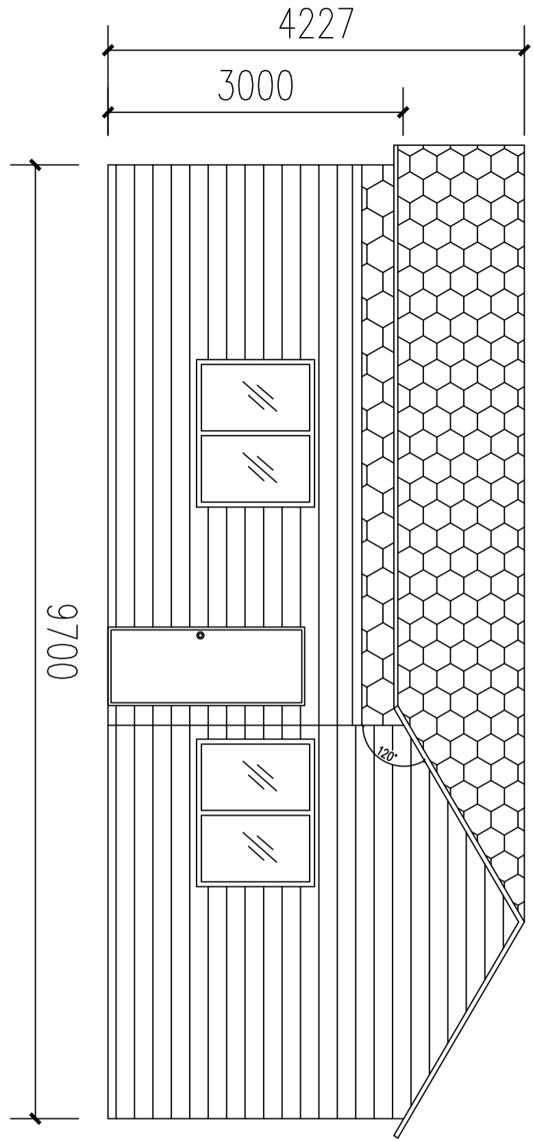
Front elevation
